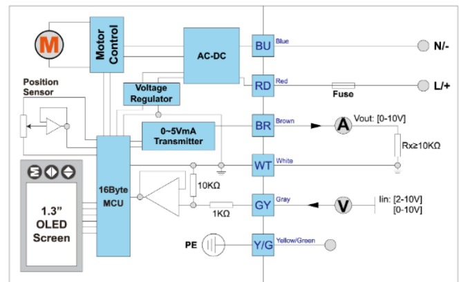
SCHEMA 0-10V
