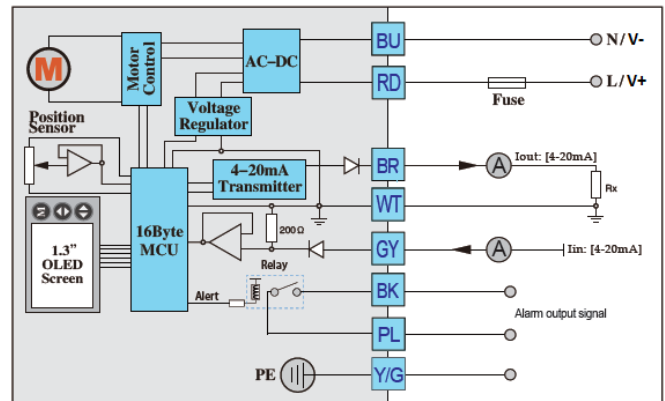
SCHEMA 4-20mA
