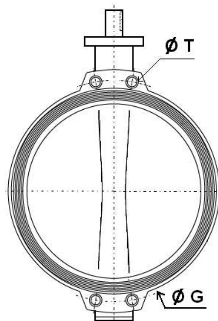
DN450-600
