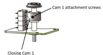
CLOSING CAM ADJUSTMENT
