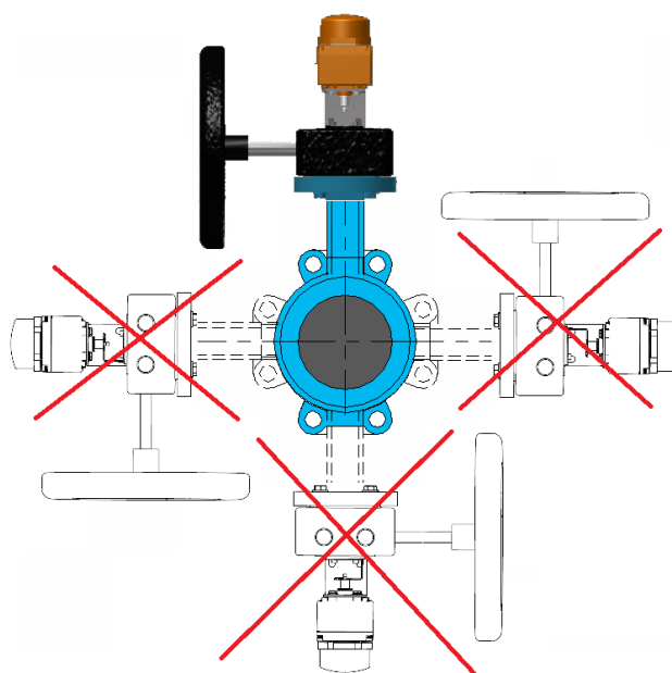
DN200 - DN400
